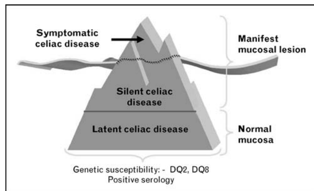
Figure 1 The celiac iceberg
