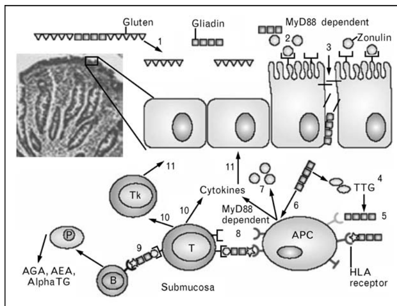
Figure 2 Proposed role of abnormal intestinal permeability in the pathogenesis of celiac disease (reproduced from [28*])
